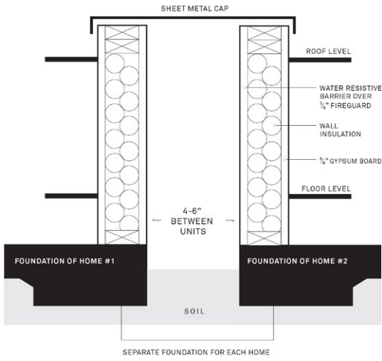
Cross Section of Airspace Separating Homes
